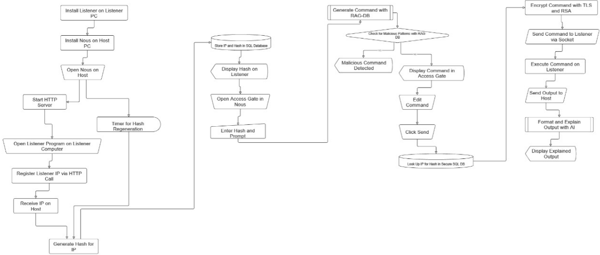
Figure 1: System Workflow
